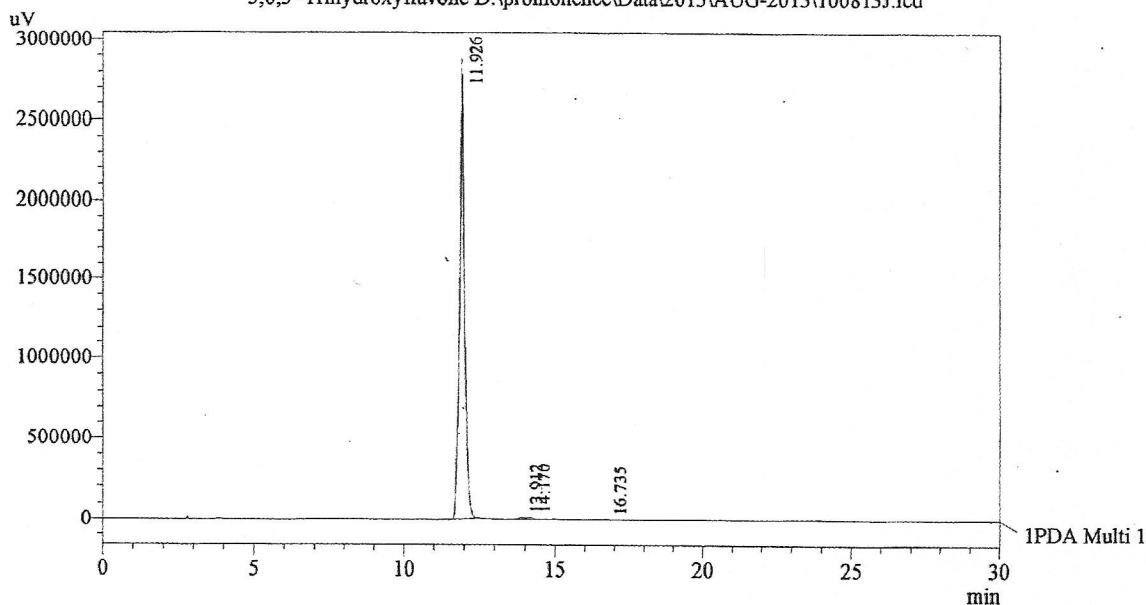
Chromatogram 3,6,3'-Trihydroxyflavone D:\promonence\Data\2013\AUG-2013\100813J.lcd
